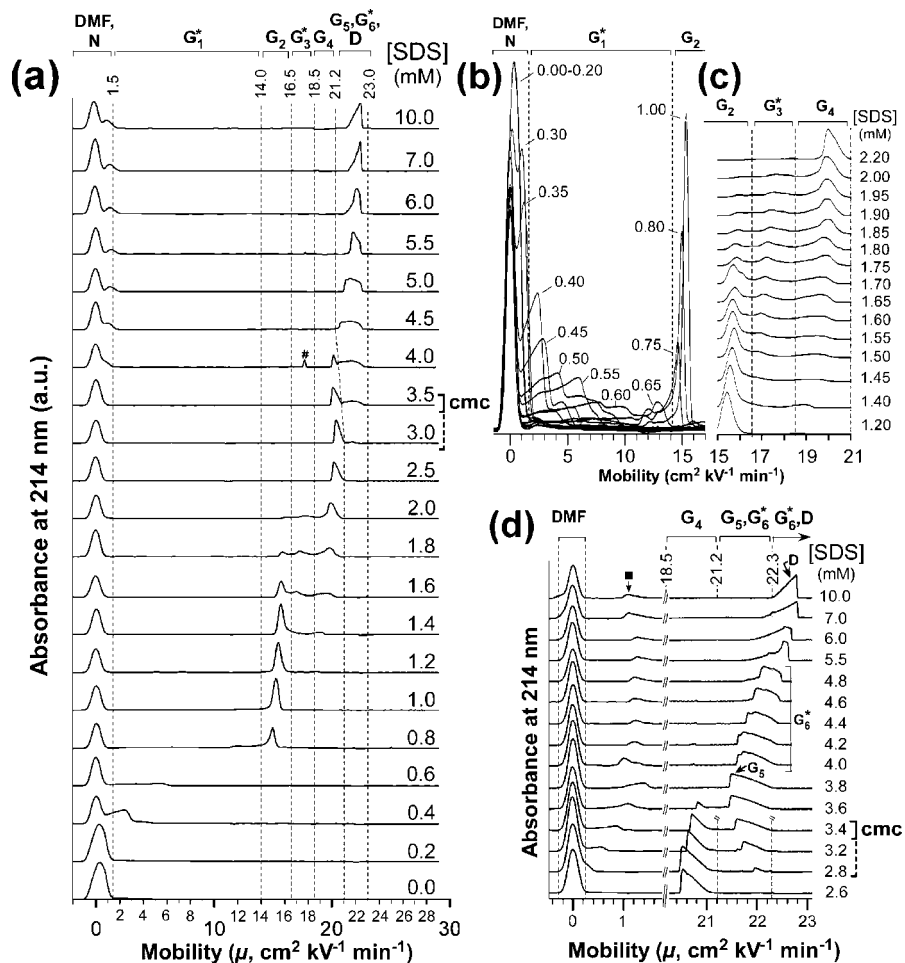
Figure 1. (a) Electropherograms of UBI-SDS n complexes obtained after dialyzing native ubiquitin (UBI) against tris–glycine (TG) containing concentrations of SDS (from 0 to 10 mM) for 170 h. The total concentration of UBI and UBI-SDS n complexes in the injected plug is 50 μM. Capillary electrophoresis (CE) was performed with a “short” capillary (total length of 60.2 cm; length from injection to the detector of 50.0 cm), with an applied voltage of 30 kV. Each of the electropherograms is labeled with the concentration of SDS. The critical micelle concentration (cmc) of SDS in this medium is 3.4 mM, as determined by CE using 2-hydroxymethylenaphthalene (plain bracket; inferred from the results in Figure S3). The cmc is also inferred by observing the formation of a shoulder on the neutral marker peak due to an impurity, either in the presence or in the absence of proteins (dotted bracket; inferred from the results in Figure 1e (■) and Figure S3). Native UBI (e.g., N) has a net charge close to zero; the peak for N is therefore superimposed on the neutral marker DMF. The peak marked (#) was not reproducible. Dotted vertical lines represent the electrophoretic boundaries we used to define each group (G) of UBI-SDS complexes (including N and D). We used these boundaries in the thermodynamic analysis. (b,c) Electropherograms in specific regions of interest (with the “short” capillary). (d) High-resolution electropherograms of UBI-SDS complexes obtained at concentrations of SDS ranging from 2.6 to 10 mM and analyzed with a “long” capillary (total length of 110.0 cm, length to the detector of 100.0 cm).
