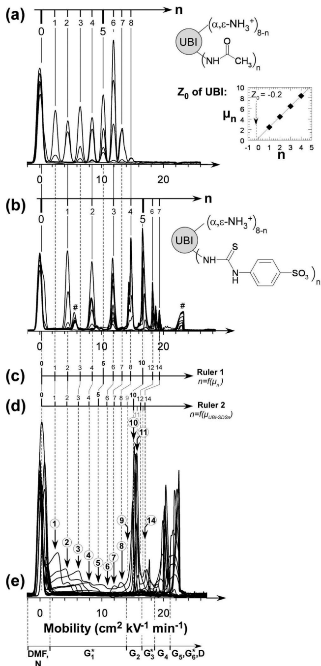
Figure 4. Superposed electropherograms of charge ladders of ubiquitin obtained respectively by acylation of \epsilon -lysine residues with (a) acetic anhydride and (b) 4-sulfophenylisothiocyanate. Peaks marked with (#) disappear after extensive dialysis. The buffer is tris-glycine, pH 8.4. The inset in panel a corresponds to the plot of the electrophoretic mobilities of the rungs of the acetyl charge ladder of UBI as a function of acetylations n and allows the determination of the net charge of native UBI as a function of charge increment upon acylation, \Delta Z . (c) Ruler 1 correlates experimental mobilities \mu_n of the rungs of a UBI charge ladder to the number of acylations n . (d) Ruler 2 correlates the corrected mobilities ( \mu_{\text{UBI-SDS}_n} , eq 4) of rungs of charge ladders to the number of acylations n . This second ruler permits the determination of the stoichiometry of UBI-SDS _n complexes in panel e. Steps in gray in Ruler 2 were extrapolated from steps in black. (e) Superposition of CE electropherograms shown in Figure 1. Labels in circles indicate the stoichiometries of UBI-SDS _n complexes within G _1 *, G _2 , and G _3 * according to Ruler 2.
