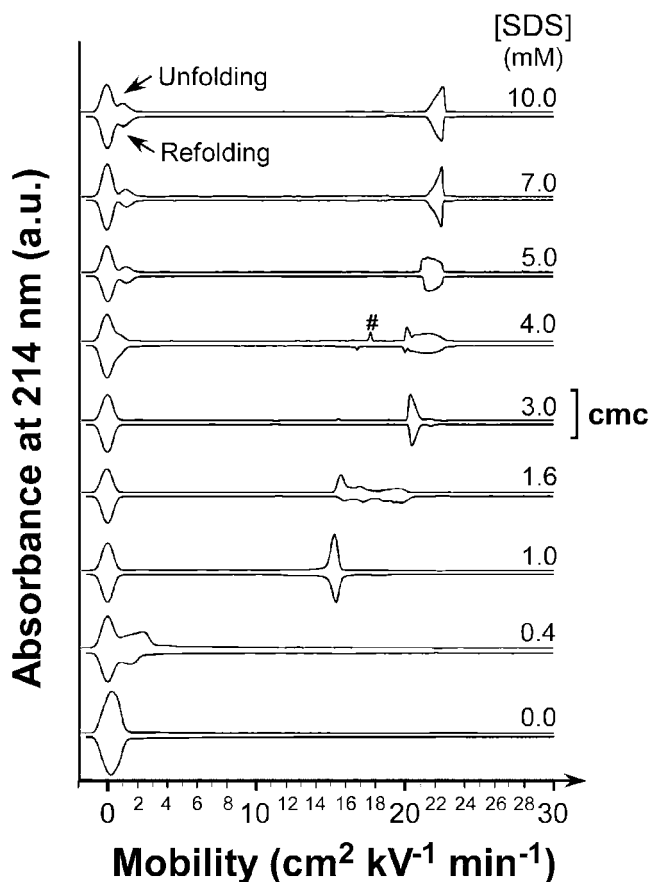
Figure 3. CE traces demonstrating reversibility and equilibrium. Electropherograms of UBI-SDS n complexes obtained after dialyzing native (N) and SDS-denatured UBI (D, incubated in 10 mM of SDS in tris-glycine buffer for 170 h prior refolding) against tris-glycine buffer containing different concentrations of SDS over 170 h. “Unfolding” experiments correspond to the dialysis of native UBI against higher SDS concentration, and “Refolding” experiments correspond to dialysis of unfolded/denatured UBI (initially in 10 mM SDS) against lower concentrations of SDS. The peak marked (#) was an artifact. Electropherograms were mirrored across the x -axis to facilitate comparison.
