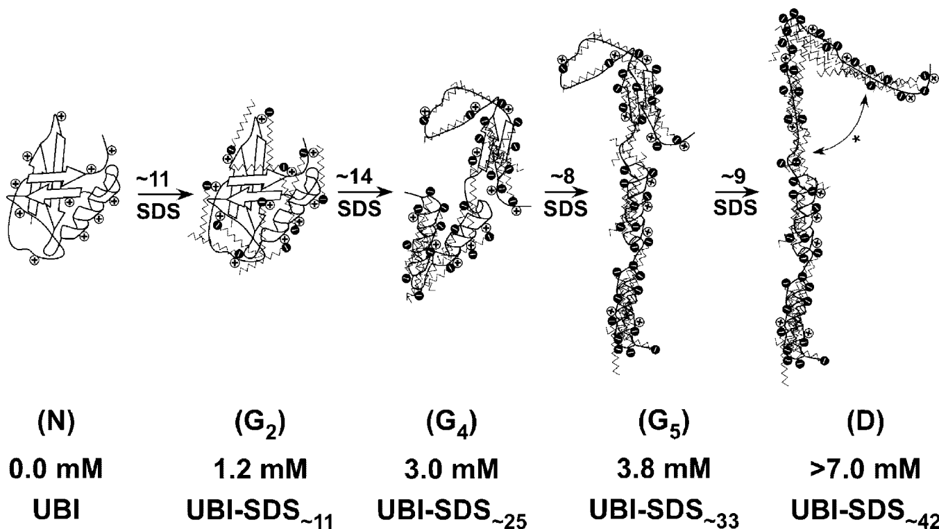
Figure 7. Pictures describing the hypothetical structure of UBI-SDS n complexes within groups N, G 2 , G 4 , G 5 , and D. The 11 cationic sites (e.g., 7 lysines and 4 arginines; we consider the unique histidine and the amino N -terminus to be uncharged at pH 8.4) are represented by positive charges along the protein backbone. N represents the native UBI (PDB 1UBQ; one turn of the \alpha -helix contains four amino acids). G 2 is a native-like UBI-SDS complex (as revealed by CD, Figures 2a,b and S4a) associated with 11 bound SDS molecules (as determined from the charge ladder analysis, Figure 4e). G 4 is less organized (perhaps a molten globule, Figure 2c), obtained after the binding of \sim 14 SDS to G 2 (cf. Figure 6b) with the conversion of about half of the \beta -stands into \alpha -helices (cf. Figure 2b). Transitions from G 4 to G 5 and from G 5 to D respectively involve \sim 8 and \sim 9 molecules of SDS (cf. Figures 5 and 6b) with no major change in secondary structure as revealed by CD; however, D might be best represented by an unfolded, SDS-saturated polypeptide with extensive \alpha -helical structure, represented in this cartoon by the disruption of the remaining \beta -strand in G 5 (*).
